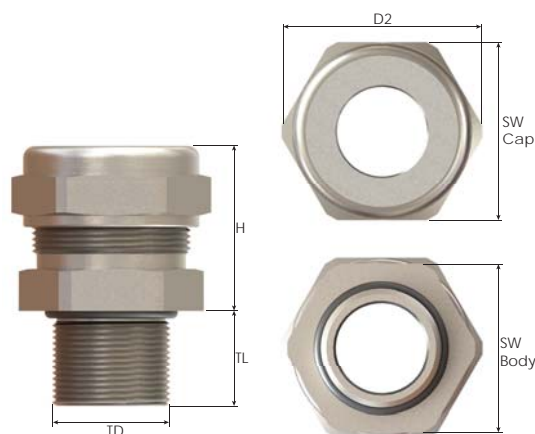
Thread Type METRIC acc. to ISO 965-3
